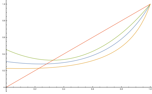
Figure 9: The graphs of f for p = 1/2 (blue), p = 1/4 (orange), p = 9/10 (green)
