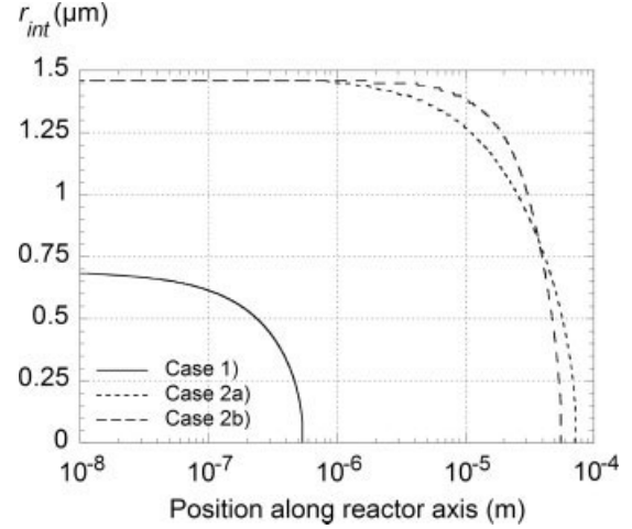
Figure 6. Position of the air/liquid interface radius along the column axis for the three scenarios of precipitation— Fv_a = 4.7 \text{ m}^3/\text{h STP} .
