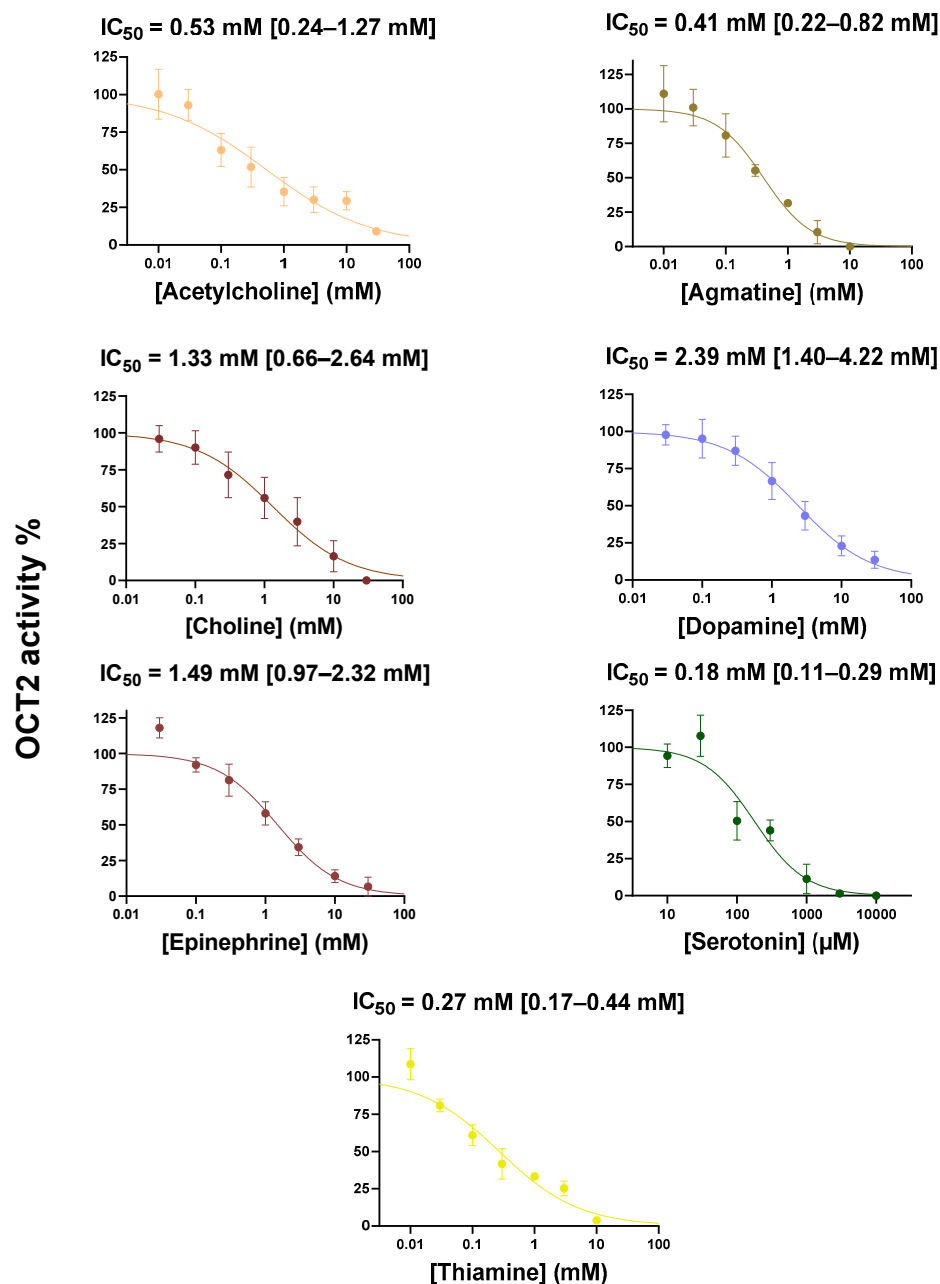
Figure 2. Cis -inhibition of OCT2 activity by endogenous OCT2 substrates. HEK-OCT2 cells were incubated with 10 \mu M DiASP, used here as a tracer substrate for OCT2, for 5 min at 37 ^{\circ} C, in the absence or presence of various concentrations of endogenous OCT2 substrates. Intracellular accumulation of DiASP was next determined by spectrofluorimetry and normalized to protein content. Data are expressed as % of OCT2 activity found in untreated control cells, arbitrarily set at 100%; they are the means \pm SEM of at least three independent experiments performed in quadruplicate. IC_{50} values and 95% confidence intervals are indicated on the top of graphs.
