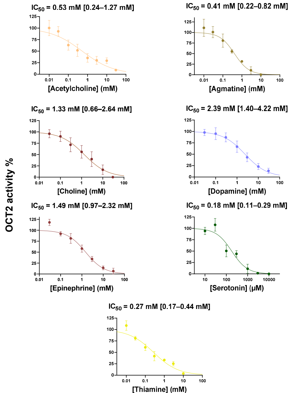
Figure 2. Cis -inhibition of OCT2 activity by endogenous OCT2 substrates. HEK-OCT2 cells were incubated with 10 μM DiASP, used here as a tracer substrate for OCT2, for 5 min at 37 °C, in the absence or presence of various concentrations of endogenous OCT2 substrates. Intracellular accumulation of DiASP was next determined by spectrofluorimetry and normalized to protein content. Data are expressed as % of OCT2 activity found in untreated control cells, arbitrarily set at 100%; they are the means ± SEM of at least three independent experiments performed in quadruplicate. IC 50 values and 95% confidence intervals are indicated on the top of graphs.
