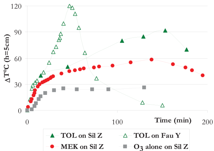
Figure 7. Temperature profiles inside the bed during ozonation at 18 g/m 3 of pure and VOC saturated zeolite
