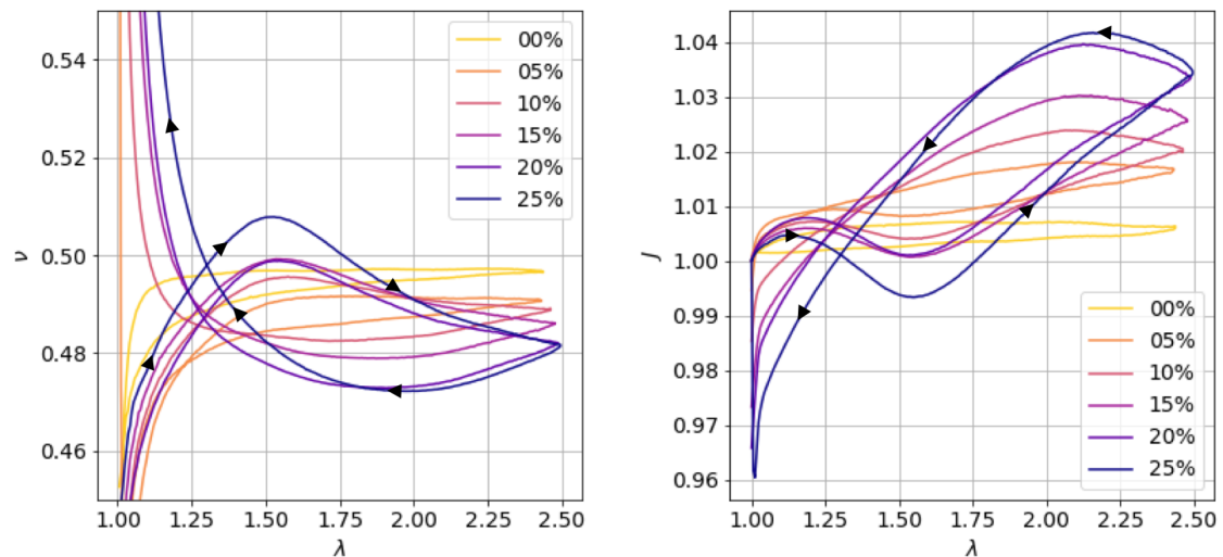
Figure 8: Poisson ratio \nu (left) and change in volume J (right) vs. extension. The loading-unloading path is shown by the black arrows.
