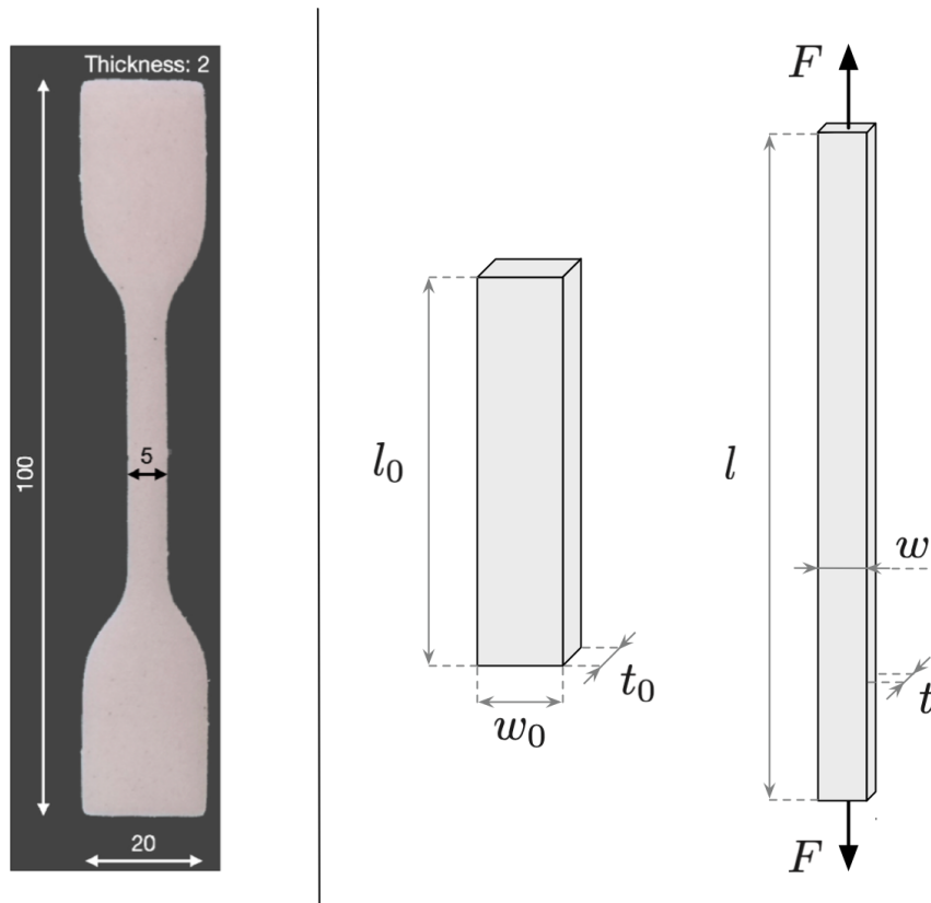
Figure 1: Sample. Left: dimensions (mm). Right: notations.
