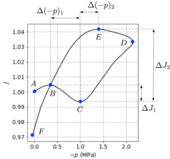
Figure 9: Volumetric response of the six materials.
