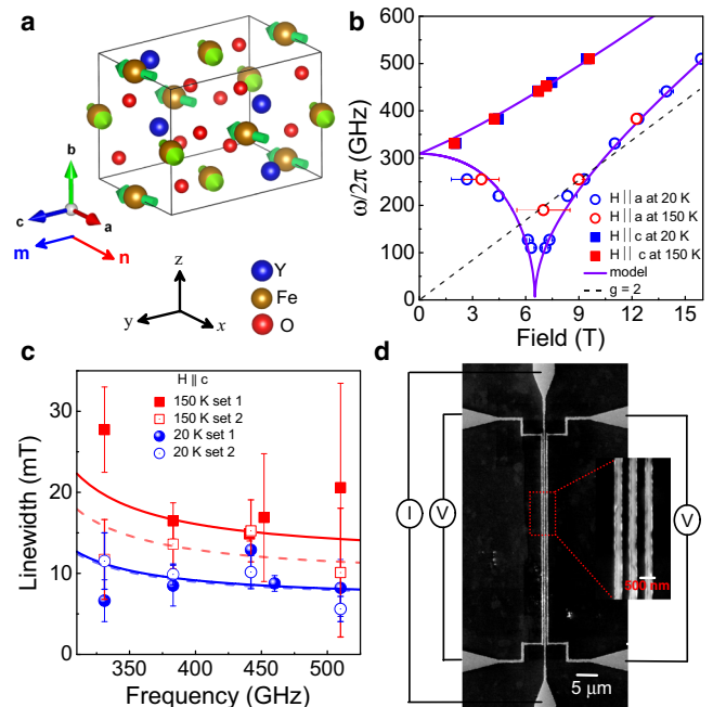
Fig. 1 | Crystal structure, magnetic resonance and the device. a Crystal structures of \text{YFeO}_3[010] , where the nearest neighbour Fe-ions are coupled antiferromagnetically along the easy-axis ( [100] a -axis) and the moments are slightly canted along the c -axis which yield a net weak magnetization directed parallel to the c -axis. The arrows in the structure indicate the direction of spins of the Fe ions. b Resonance frequency as a function of magnetic field along a -axis (open symbol) and c -axis (closed symbol) for two different temperatures, 20 K in blue and 150 K in red. The model parameters for the fits are \mu_0 H_E = 635\text{ T} , \mu_0 H_a = 0.19\text{ T} , \mu_0 H_b = 0.77\text{ T} and \mu_0 H_{DMI} = 12\text{ T} . The g = 2 line shows the frequency of a potential spurious paramagnetic resonance. c Linewidth as a function of frequency for the configuration of H along c -axis at 20 K and 150 K. The open and closed symbols correspond to data taken separately, after removal and reintroduction of the sample, to test reproducibility. The solid solid and dashed lines are the theoretical fitting using the model from Fink 42 , which yields damping coefficients of 3.5 \pm 0.4 \times 10^{-6} and 3.4 \pm 0.3 \times 10^{-6} for the two sets of data at 20 K and 6.2 \pm 0.3 \times 10^{-6} and 4.6 \pm 0.5 \times 10^{-6} for 150 K. The extracted parameters from (b), \mu_0 H_E , \mu_0 H_a , \mu_0 H_b and \mu_0 H_{DMI} are used in this model. d SEM image of a typical device, where the charge current is driven along the middle wire and the non-local voltages are measured in both wires to the left and right of it. We associate orthogonal coordinates with the crystallographic axes: x \parallel a , y \parallel c , z \parallel b .
