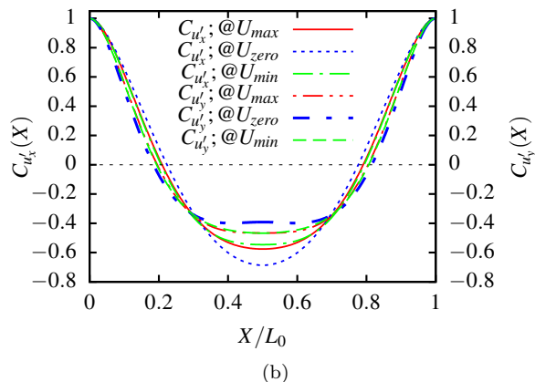
FIG. 4. Normalized temporal (a) and spatial (b) autocorrelation functions of u'_x (left axes) and u'_y (right axes). In both (a) and (b) data from probes where the mean flow is maximum, zero and minimum are shown. The Weissenberg number is Wi = 24.9 .
