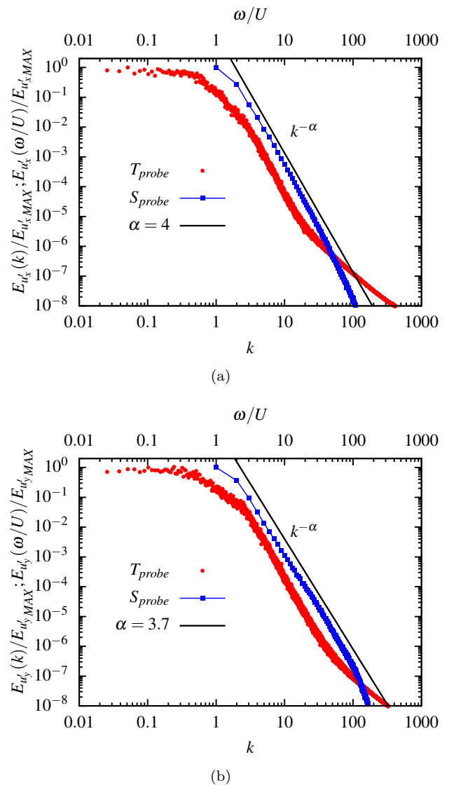
FIG. 9. Spectra of velocity fluctuations u'_x (a) and u'_y (b) from temporal and spatial data from probes located where the mean flow is maximum and minimum, for Wi = 24.9 . The bottom horizontal axis refers to the spatial spectra, the top one refers to temporal spectra, after conversion, where \omega = 2\pi f , f is the frequency and U the mean flow intensity. All spectra in (a) and (b) are normalized by their maximum values.
