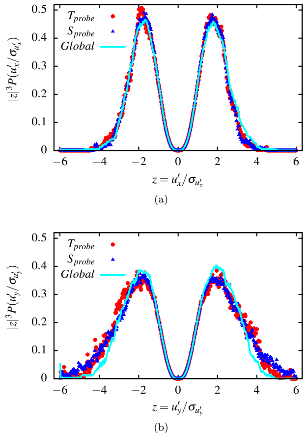
FIG. 7. Third-order statistics |z|^3 P(z) for z = u'_x / \sigma_{u'_x} (a) and z = u'_y / \sigma_{u'_y} (b), for Wi = 24.9 . Red (circle) and blue (triangle) points respectively correspond to data from temporal and spatial probes, located where the mean flow is maximum and minimum; aqua color points (solid line) correspond to global spatial data. All spatial statistics are further averaged over time using 1000 instantaneous velocity fields.
