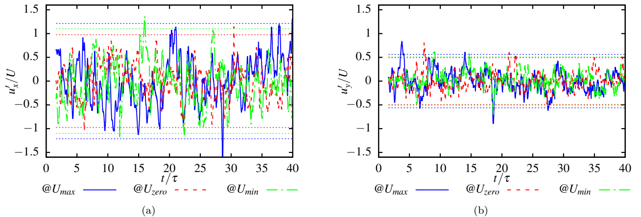
FIG. 3. Time series of u'_x (a) and u'_y (b), normalized by the mean flow amplitude \overline{U} , at Wi = 24.9 , as recorded by three different probes at the U_{max}, U_{zero}, U_{min} locations. Horizontal dotted lines indicate \overline{u'_{x,y}} \pm \sigma_{u'_{x,y}} , where the overbar denotes a temporal average and \sigma_{u'_{x,y}} the standard deviation with respect to it. To ease visualization, only a short subset of the full data set (which reaches t/\tau = 800 ) is shown.
