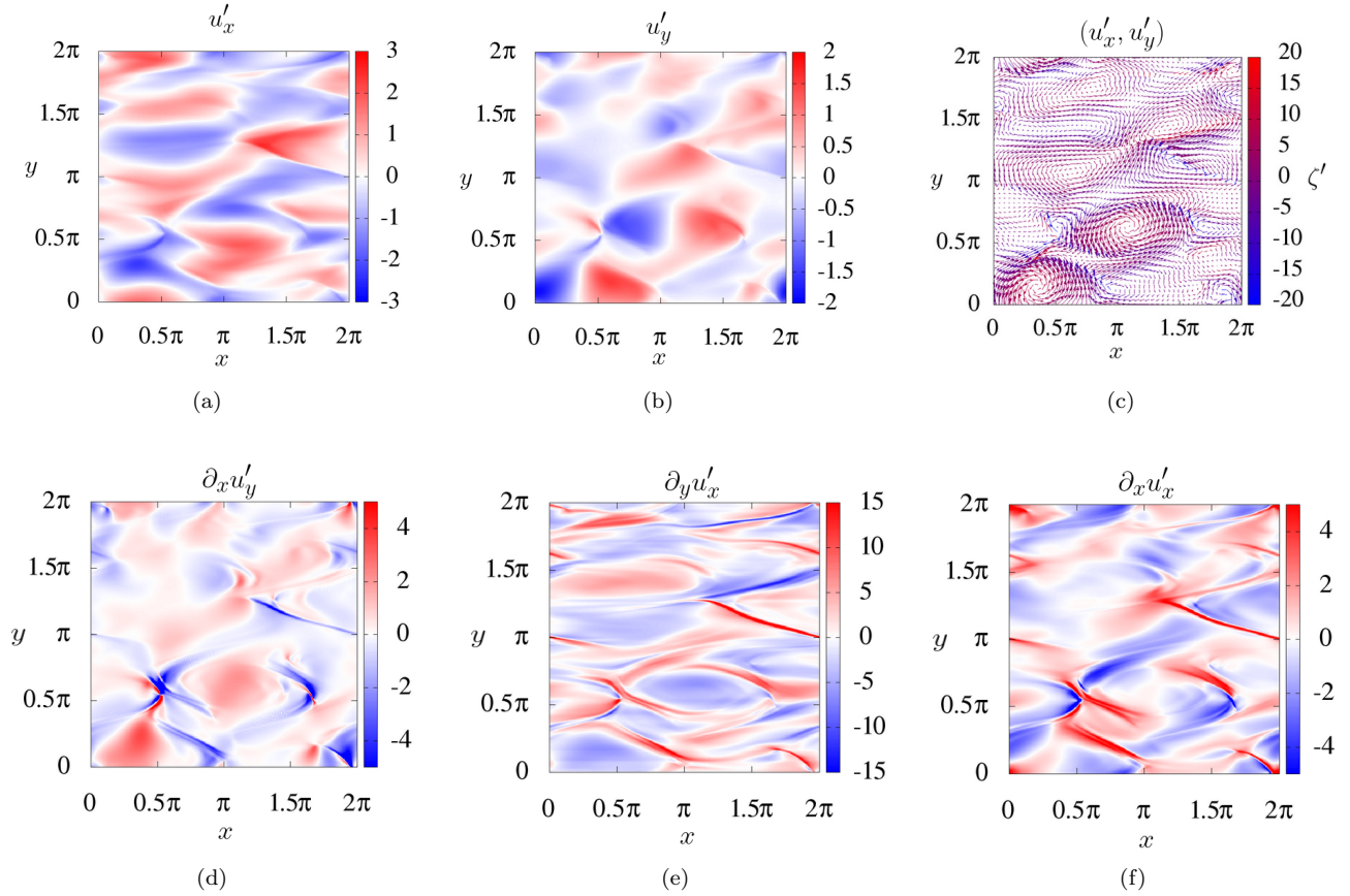
FIG. 2. Instantaneous snapshots of u'_x(x, y) (a), u'_y(x, y) (b), \partial_x u'_y (d), \partial_y u'_x (e), \partial_x u'_x (f). Panel (c) shows the vector-field representation of the fluctuating velocity \mathbf{u}' at the same instant of time as the other panels; here the color codes the intensity of the fluctuating vorticity \zeta' .
