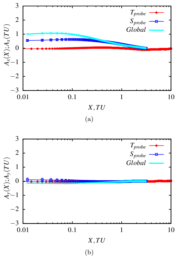
FIG. 12. Scale-dependent skewness A_i = S_{u'_i}^{(3)}(X) / [S_{u'_i}^{(2)}(X)]^{3/2} versus the spatial increment (either measured directly, X , or via the mean flow intensity, TU ). Panel (a) refers to u'_x , panel (b) refers to u'_y . Red (circle) and blue (square) points respectively correspond to data from temporal and spatial probes, located where the mean flow is maximum and minimum; aqua color points (solid line) are for global statistics. All spatial statistics are further averaged over time using 1000 instantaneous velocity fields. For all the data shown the error bar, estimated by dividing the data sets into two equal parts, is of the order of the point size.
