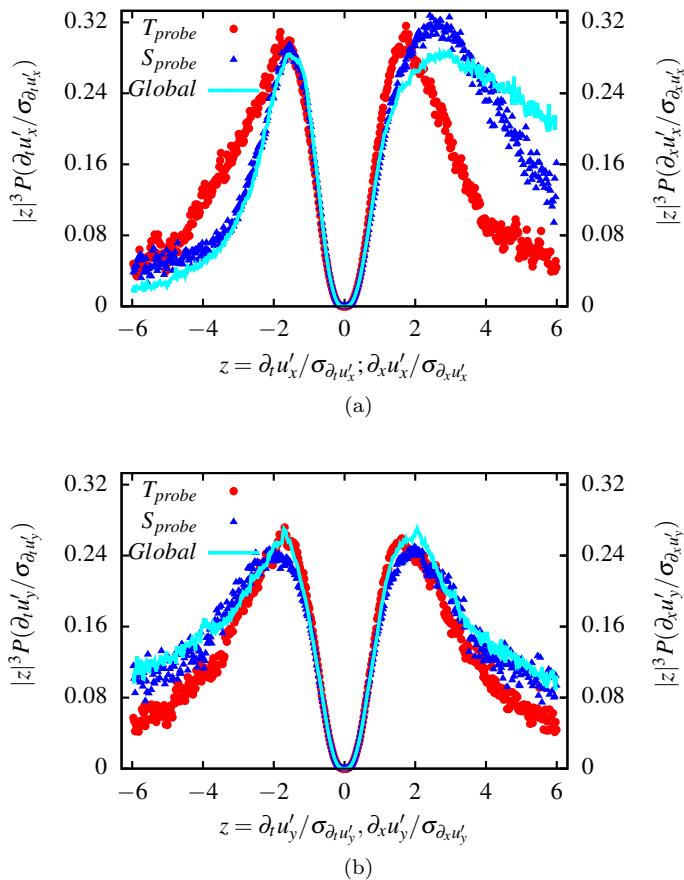
FIG. 8. Third-order statistics |z|^3 P(z) for z = \partial_i u'_i (local accelerations) and z = \partial_x u'_i (longitudinal gradients), for Wi = 24.9 . Panel (a) refers to the streamwise velocity component ( i = x ), panel (b) to the cross-stream one ( i = y ). Red (circle) and blue (triangle) points respectively correspond to data from temporal and spatial probes, located where the mean flow is maximum and minimum; aqua color points (solid line) correspond to global spatial data. All spatial statistics are further averaged over time using 1000 instantaneous velocity fields.
