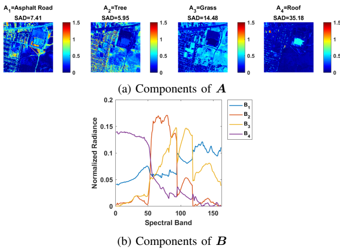
Fig. 19: Urban. NMF results of the HSI matrix for R = 4
