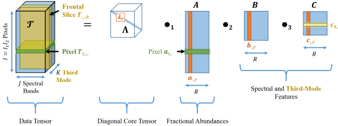
Fig. 2: Canonical polyadic decomposition of a third-order tensor. The tensor is formed of K matricized HSIs that are stacked along the third mode. A frontal slice T_{:, :, k} (in yellow) represents a matricized HSI and is associated with one row of C . A horizontal (pixel) slice T_{i, :, :} (in green) represents a matrix of features and is associated with one row of A .
