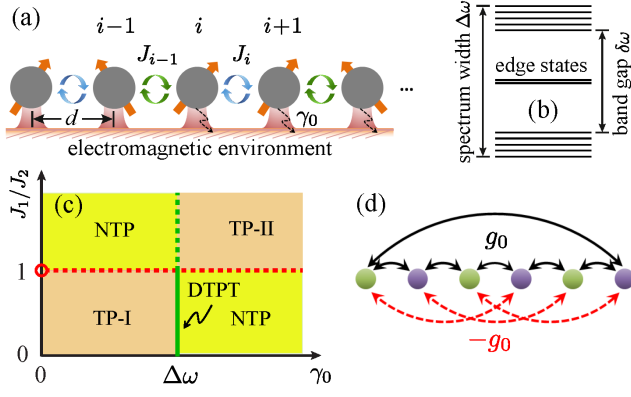
FIG. 1. (a) Schematic of a topological emitter array coupled to an electromagnetic environment. Emitters have nearest-neighbor interactions J_i , homogeneous spacing d , and decay rate \gamma_0 to the environment. (b) Single-excitation spectrum of the topological system with spectrum width \Delta\omega and bandgap \delta\omega . (c) Phase diagram of the system for emitter spacing d = 3\lambda_0/4 . There are topological phases TP-I (having edge states), TP-II (having no edge state) and non-topological phase (NTP). The red circle at (\gamma_0 = 0, J_1/J_2 = 1) represents the original phase transition in the SSH model. The horizontal red-dashed line denotes the SSH-type phase transition in the dissipative regime. The vertical green line represents the environment-induced topological phase transition where the decay rate \gamma_0 is equal to the spectrum width \Delta\omega of the topological system. In particular, the green-solid line indicates the dissipative topological phase transition. (d) Photon-mediated interactions H_{ph} for d = \lambda_0/4 ( g_0 = \gamma_0/2 ) and d = 3\lambda_0/4 ( g_0 = -\gamma_0/2 ).
