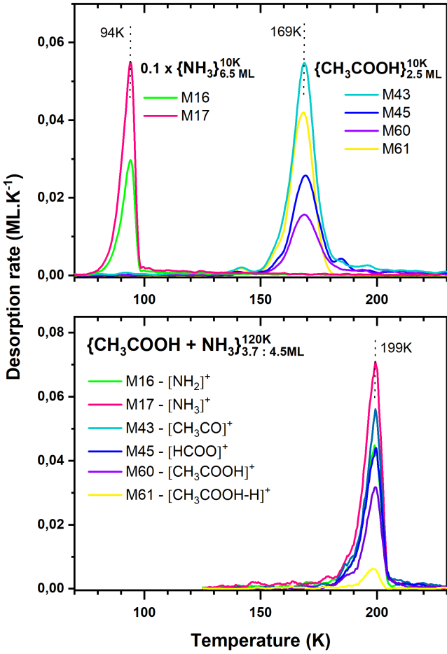
Fig. 5. TPD spectra of experiments involving ammonium acetate. Top panel: TPD spectra of \text{NH}_3 and \text{CH}_3\text{COOH} . Bottom panel: TPD spectrum of \text{NH}_4^+\text{CH}_3\text{COO}^- ; the sharp profile of the desorption is linked with a high pre-exponential factor and may indicate that the dissociation of the salt is at the origin of the desorption process.
