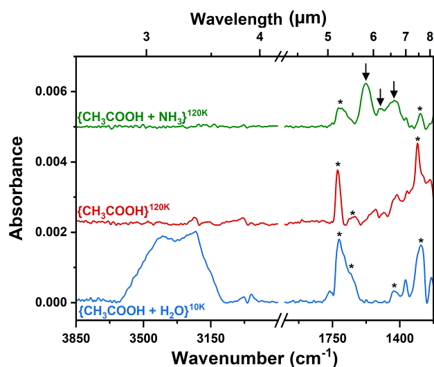
Fig. 4. RAIRS spectra of experiments involving the formation of ammonium acetate. The highlighted bands using stars are related to absorption features of neutral acetic acid. When \text{NH}_3 and \text{CH}_3\text{COOH} are co-deposited, the bands related to \text{NH}_4^+\text{CH}_3\text{COO}^- appear (indicated by arrows.)
