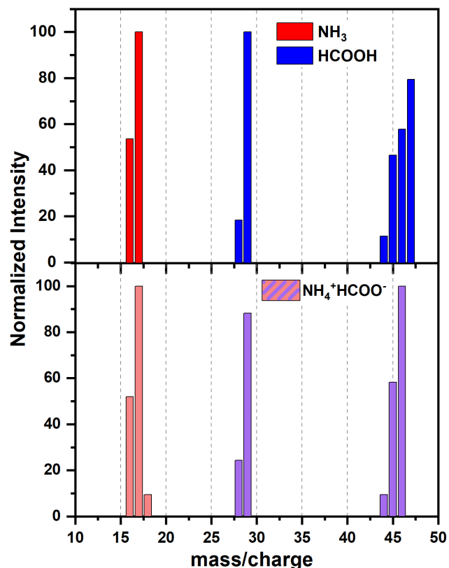
Fig. 3. Mass spectra of NH 3 , HCOOH, and NH 4 + HCOO - . Intensities are normalized to the most intense of the peaks for NH 3 ( m/z = 17 ) and HCOOH ( m/z = 29 ). For NH 4 + HCOO - the fragments corresponding to ammonia are normalized to the most intense of the peaks ( m/z = 17 ) and those from formic acid to the second most intense peak ( m/z = 46 ).
