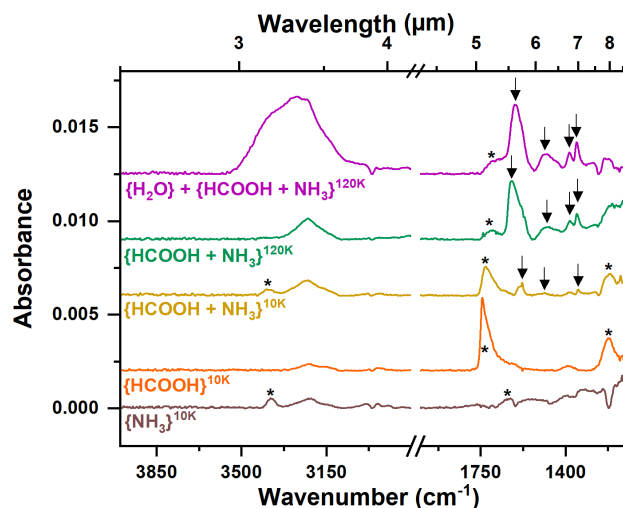
Fig. 1. RAIRS spectra of experiments related to the formation of ammonium formate. The bands highlighted by stars (*) correspond to the absorption features of the neutral molecules \text{NH}_3 and \text{HCOOH} . When these two species are co-deposited, vibrations of the molecular ions ( \text{NH}_4^+ and \text{HCOO}^- ) appear (↓), suggesting the formation of ammonium formate.
