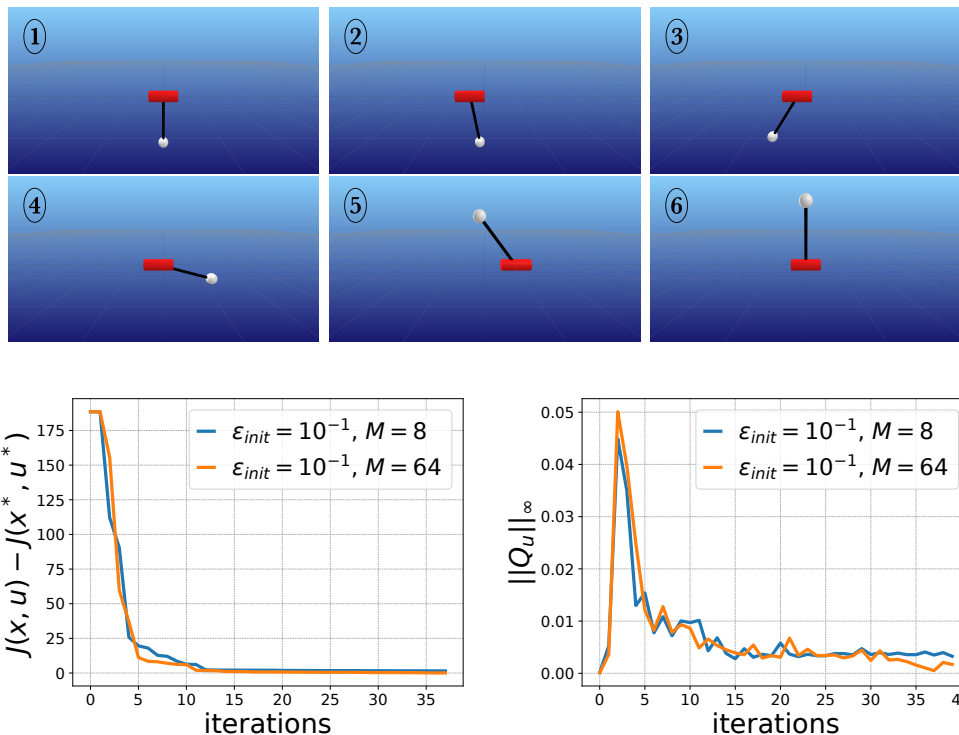
Figure 5: Top: Application of RDDP to precisely control a cartpole movement requiring overcoming dry friction on the joints and moving the pole straight upward. Bottom: Using RDDP for the cartpole task, we compare the influence of the sample size on the solution. Only a few samples (here M=8 ) are necessary to get reasonable results. Increasing the number of samples in the first order Monte-Carlo estimator of the gradients leads to very marginal improvement.
