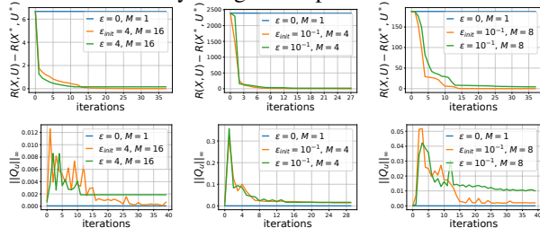
Fig. 6: Left: Randomized smoothing allows to solve tasks requiring to break contacts such as the one from Fig. 2 (Top) Middle: Complex systems such as an inverted double pendulum Right: or cartpole with dry frictions on the joints.
