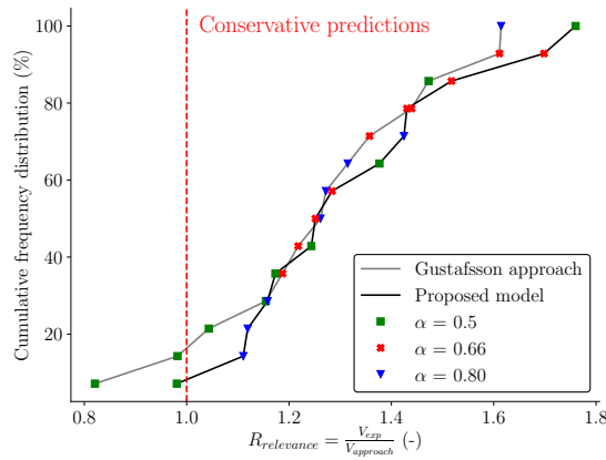
Figure 13: Cumulative frequency distribution of the relevance ratio ( R_{relevance} ) for the proposed model and the Gustafsson's approach
