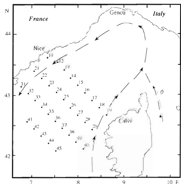
Fig. 1 Region studied of Trophos-2 (22 April to 7 May) and position of sampling sites. Arrows indicate current flow general direction
