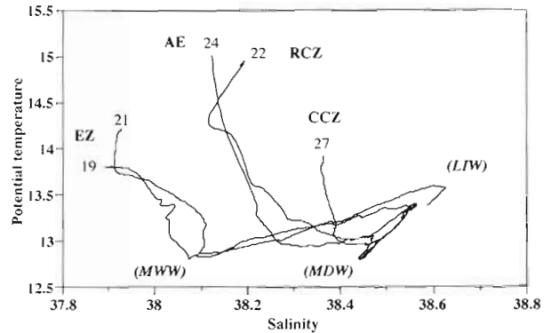
Fig. 4. Potential temperature ( ^{\circ}\text{C} )/salinity diagrams for some selected stations of the 4 hydrological zones: EZ: external zone; Stns 21, Riviera and 19, Corsica; RCZ: Riviera coastal zone; AE: anticyclonic eddy; and CCZ: Corsica coastal zone. Position of type waters: MWW: Mediterranean Winter Water; LIW: Levantine Intermediate Water, and MDW: Mediterranean Deep Water
