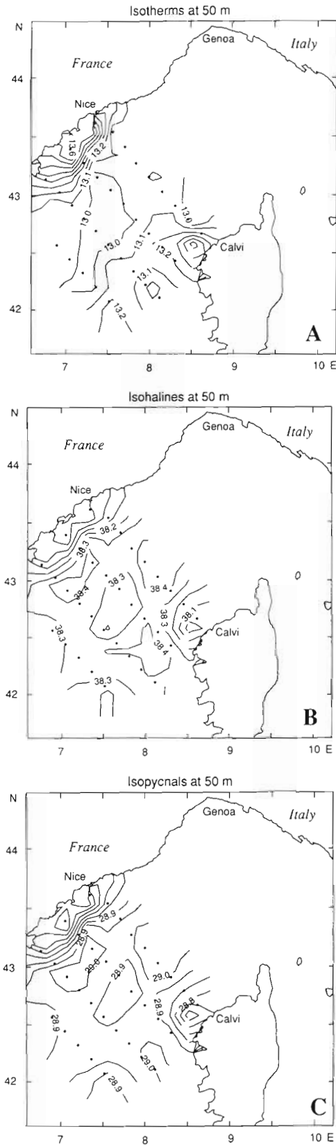
Fig. 3. Horizontal maps of (A) temperature ( ^{\circ}\text{C} ); (B) salinity; and (C) density excess ( \text{kg m}^{-3} )
