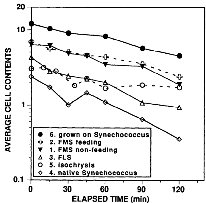
Fig. 3. Time-course changes in the average number of prey items per cell. For each prey type, a population of ciliates was exposed to the prey item, diluted at 1 : 100, and time-course samples were examined to estimate average cell contents. Numbers in the key refer to the experiment number. Estimated digestion parameters are given in Table 1.
