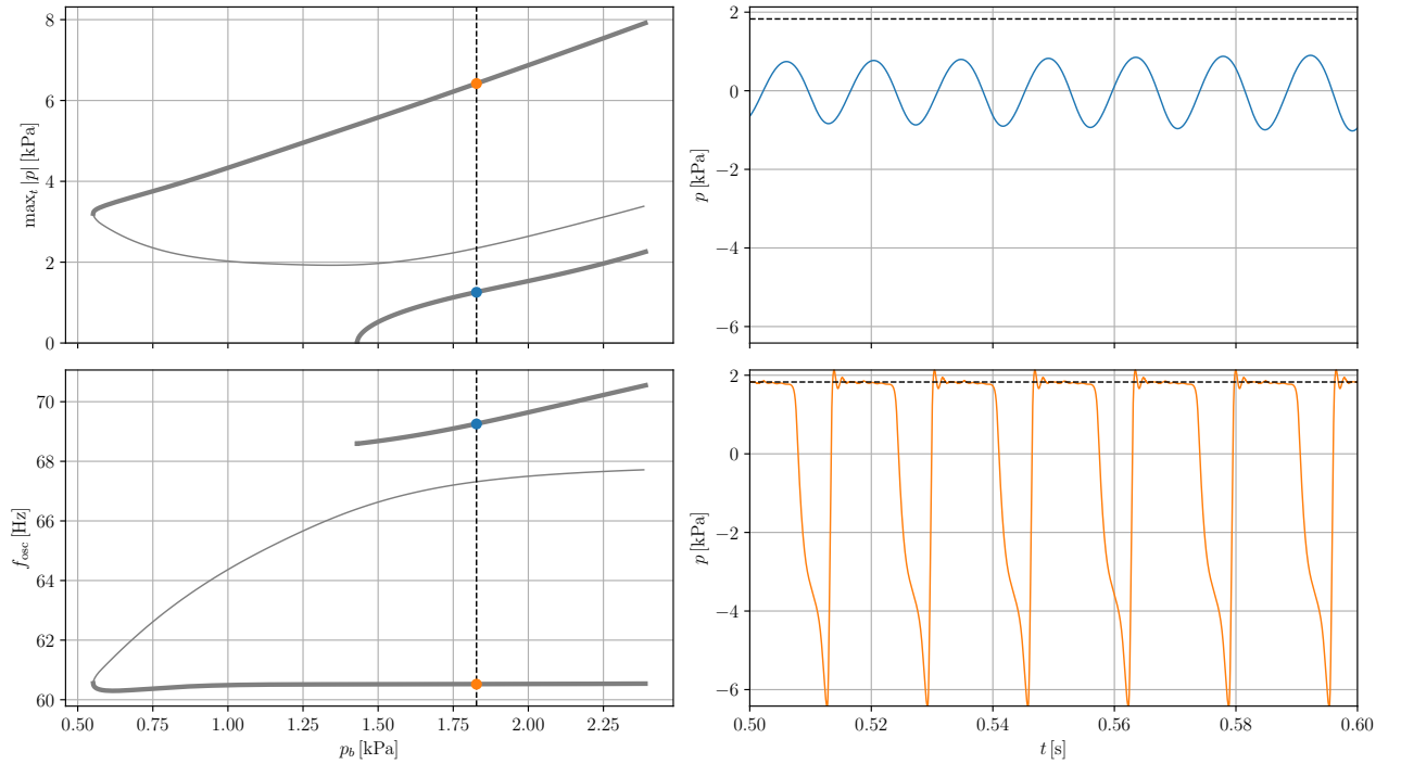
Figure 10: Typical bifurcation diagrams (left) and time-domain simulations (right) in the case of the euphonium’s first regime, obtained for p_m = 1.8 kPa and f_\ell = f_{\ell, \text{PN}}^{\text{opt, per}} (Pedal Note) = 49 Hz. Left plots represent the maximum amplitude of the periodic oscillation branches vs. the blowing pressure (top) and the frequency of the corresponding periodic solutions vs. the blowing pressure (bottom). The line thickness indicates whether the branch portion is stable (thick line) or unstable (thin line). Right plots represent the time evolution of the acoustic pressure at two points of the bifurcation diagrams above, given by the intersection of the vertical dotted line and the branches. Top: time-domain simulation of the ghost note (blue point on the bifurcation diagrams); bottom: time-domain simulation of the pedal note (orange point on the bifurcation diagrams). The horizontal dotted line represents the value of p_m .
