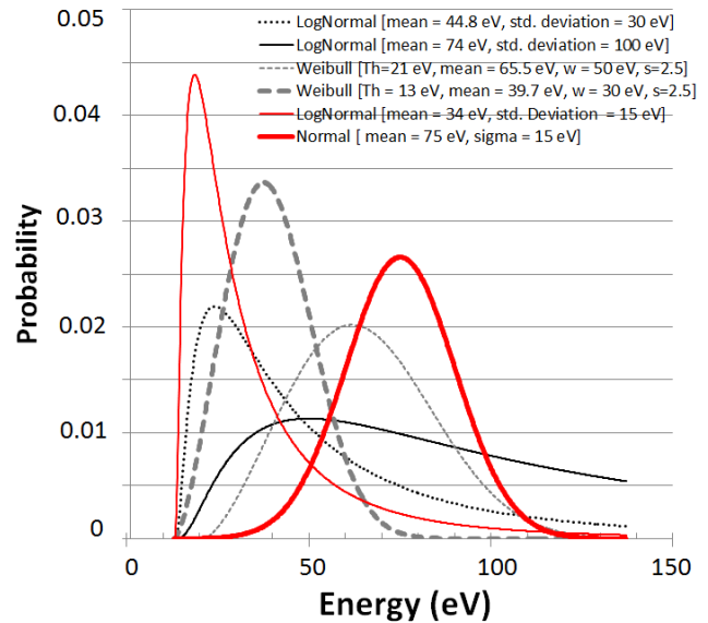
Fig. 10. Comparison of different damage energy distribution probability normal (mean = 75 eV, Std. Dev. = 15 eV), LogNormal (mean = 74 eV, 44.8 eV, 34 eV, Std. Dev. = 100 eV, 30 eV, 15 eV), Weibull distribution (th=13 eV, 21 eV, w = 30 eV, 50 eV and s = 2.5).
