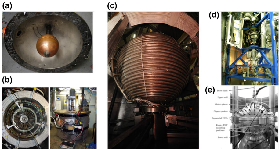
Fig. 8 The hydromagnetic spherical Couette experiments: a–c the three Maryland experiments—30 cm, 60 cm, and 3 meter, respectively ( Sources : S.A. Triana, Kelley 2009 and D. Lathrop). d DTS experiment (picture courtesy: H.-C. Nataf) and e HEDGEHOG experiment (figure from Kasprzyk et al. 2017). See also online movies of the 3-meter setup at https://youtu.be/bm_iqzmR2cE and https://youtu.be/rAYW9n8i-C4
