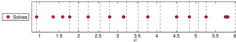
Figure 2: The points \tilde{\mu} \in \mathcal{S}_k , k = 1, \dots, K for which the solutions u(\tilde{\mu}) have been computed. The dotted vertical lines indicate the boundary of the subdomains \mathcal{D}_k , k = 1, \dots, K (thus each interspace between two dotted vertical lines corresponds to a subdomain).
