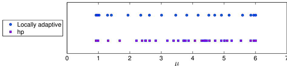
Figure 1: The J = 20 parameter points selected by the locally adaptive algorithm [3] and the 34 parameter points selected by the hp algorithm [4]. Both algorithms applied to \psi^{\text{ns}}(\cdot; \mu) with Q = 7 and prescribed tolerance of 10^{-7} on the approximation error in L^\infty([0, r_{\max}] \times \mathcal{D}) norm (with r_{\max} = 2 , the diameter of the unit sphere).
