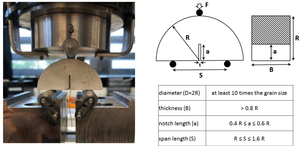
Figure 4. The new device developed at GEC laboratory for measuring the mode I fracture toughness. The sample geometry is given on the right and the requirements for the different parameters are summarized in the table.
