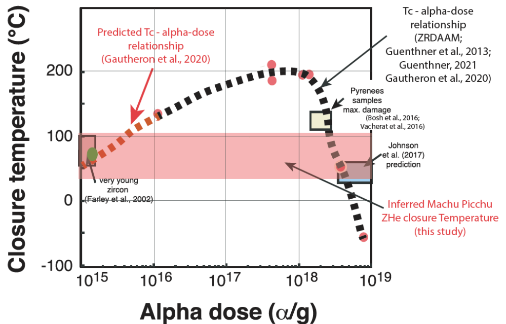
Figure 7. Update of the co-evolution of the closure temperature and the \alpha -dose (Fig. 10B of [17]) with our new data from the Machu Picchu profile (green dot). Red circles correspond to [14] data recalculated with the Density Functional Theory results (see details in [17]), the yellow box places Pyrenean samples [45,46] and the blue box represents [9] high
