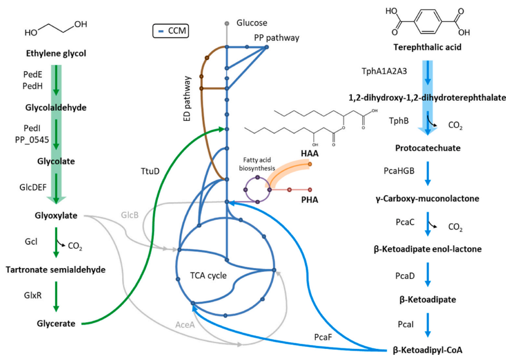
Fig. 6. Metabolic pathways for the metabolization of ethylene glycol (EG) and terephthalic acid (TA). On the left side the enzymatic steps for conversion of EG to the intermediate of the central carbon metabolism (CCM) 2-phospho-glycerate is shown (green). The grey lines represent pathways in which EG serves only as source for redox equivalents and the generation of CO 2 . On the right side the conversion of TA to the CCM intermediates succinate and acetyl-CoA is depicted (light blue). The shaded thick arrows depict reactions that have been added to the metabolic model iJN1411.
