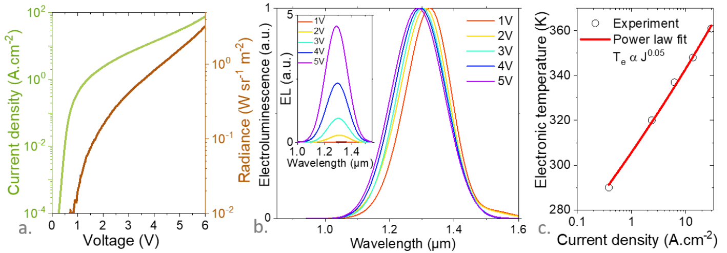
Figure 3 Performance of the \text{Hgl}_2 treated LED. a. Current density and irradiance as a function of the applied bias for the LED where the active layer is processed by a MPA and then by \text{Hgl}_2 . b. Normalized electroluminescence signals for different applied biases, highlighting a clear blue shift as the bias is increased. The inset is the non-normalized data. c. Electronic temperature as a function of the driving current of the LED.
