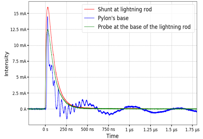
Fig. 4: Current measurements on the model pylon
