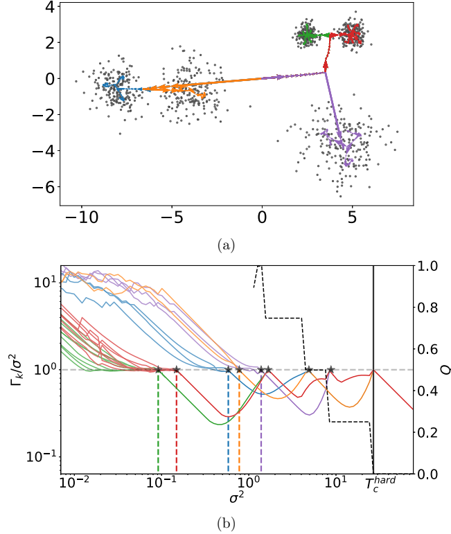
FIG. 1. (a) Displacement of K = 25 centers during the annealing procedure for a dataset with five spherical Gaussian clusters. Colors indicate in which final cluster the center ends. (b) Evolution of the ratio \Gamma_k/\sigma^2 as a function of \sigma^2 . Black stars correspond to the scales of successive transitions, the black vertical line to T_c^{\text{hard}} , and colored ones indicate the size of the clusters as defined by the maximum eigenvalue of the empirical covariance. The black dashed curve shows the evolution of Q as defined in Eq. (4) that we identify as an order parameter. This quantity is not represented for \sigma \leq 1 since the number of physical clusters K_r begins to be higher than the number of generated clusters q .
