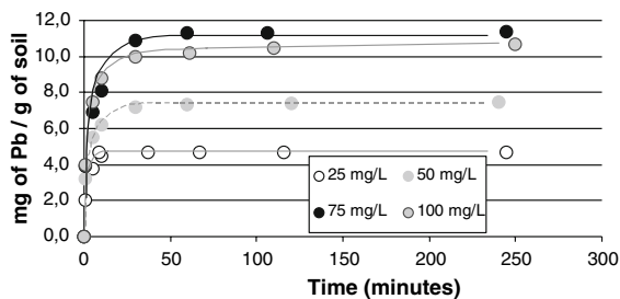
Fig. 3 Rate of Pb-immobilization in soil for initial solutions at 25, 50, 75 and 100 \text{mg Pb l}^{-1}
