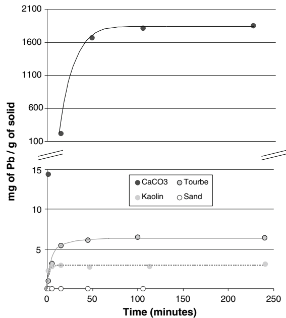
Fig. 4 Pb extraction quantity ( \text{mg Pb g}^{-1} solid), by the different constituents of the artificial soil versus time
