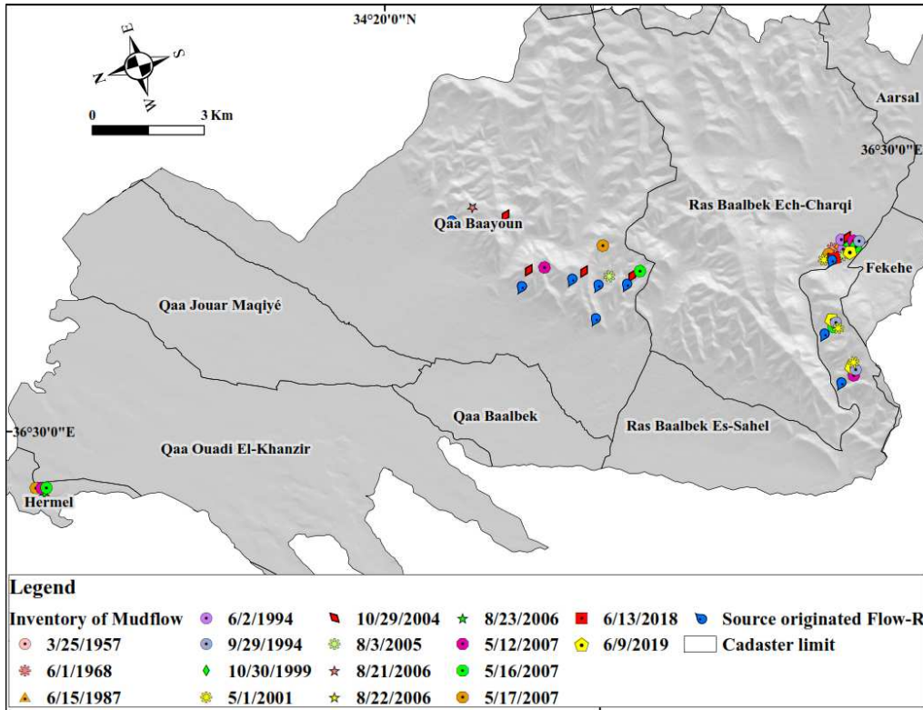
Figure 5.- Probability mudflow source map derived from the flow-R modelling in Ras Baalbek basin and inventory of Mudflow occurred in the basin from years 1957 to 2019
