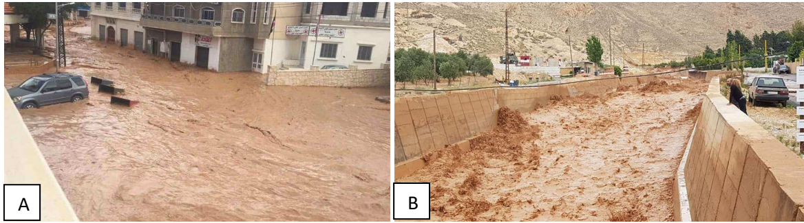
Photo 3.- A: The main road crossing the village was submerged and closed for several hours during the mudflow of June, 2018. B: the channel constructed after the sail of 1994 was flooding during the sail of June, 2018
