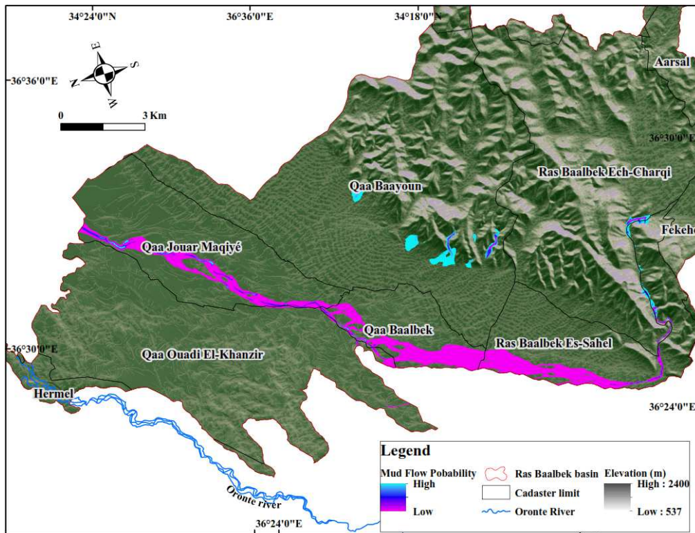
Figure 6.- Mudflow potential hazard map of the study area
