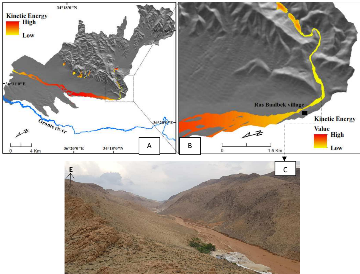
Figure 7.- Kinetic energy map derived from the flow-R modelling. A : kinetic energy map for the whole Ras Baalbek basin. B: view on the kinetic energy of the mudflow in the Ech Charqi – Ras Baalbek valley. C: photo of the sail occurred in Ech Charqi – Ras Baalbek valley on June 13, 2018
