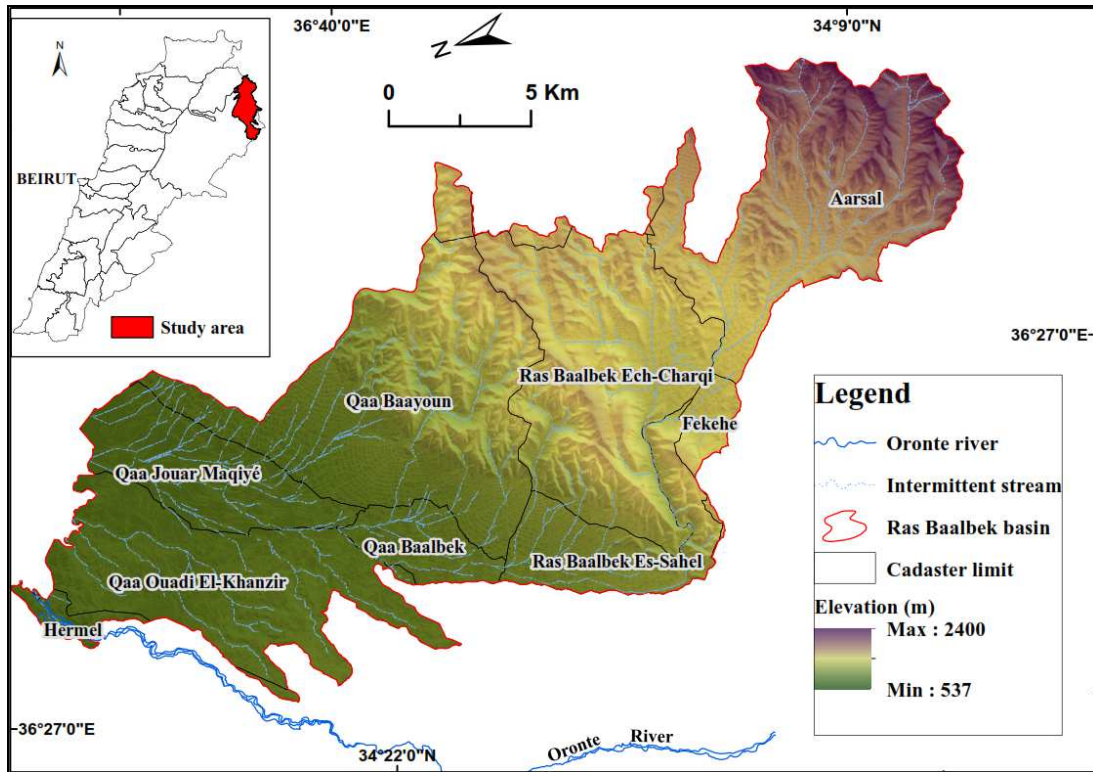
Figure 2.- Hillshade of the Ras Baalbek basin (North Bekaa)
