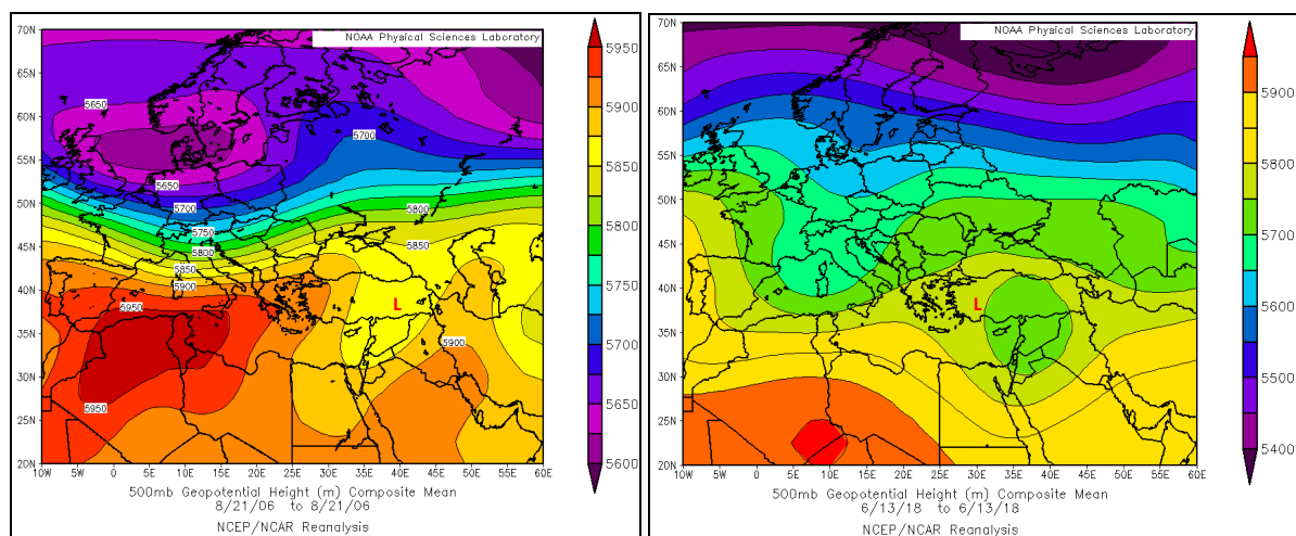
Figure 1.- Air circulation in the upper layers of the atmosphere (500 hpa) above the eastern basin of the Mediterranean that caused the cut-off lows on August 21, 2006 (to the left) and June 13, 2018 (to the right).
