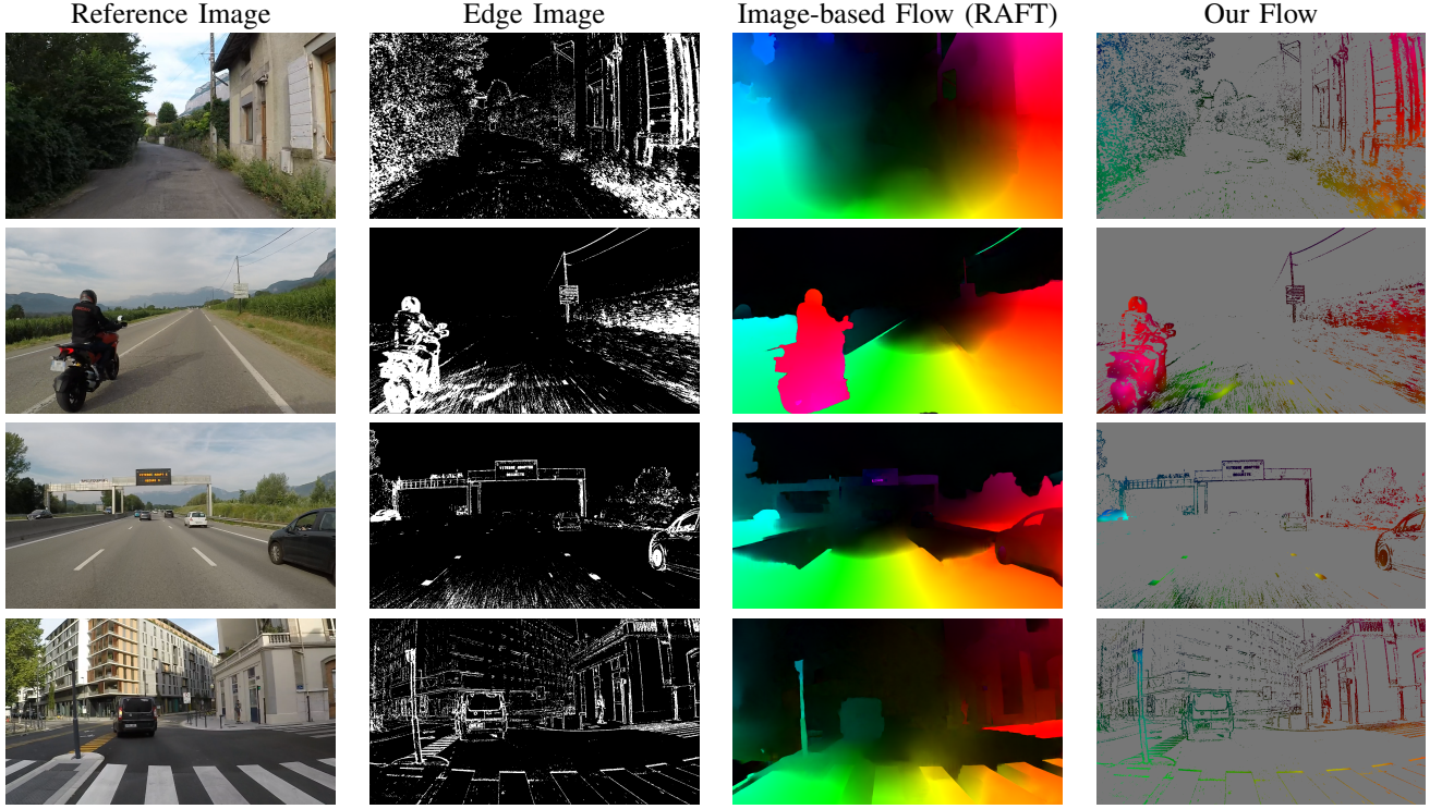
Fig. 6. Qualitative results on the 20-minute-long driving sequence. Extracts used, from top to bottom: a village street, a motorcycle overtaking, a highway, and an intersection. Best viewed in color.
