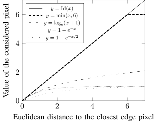
Fig. 4. Values of the distance transform as a function of the distance to the closest edge pixel. Curves represent the original distance transform, the same with an upper bound set to 6px, the natural logarithm version, and our inverse exponential formulation, with \alpha set to 1 and 2 respectively.
