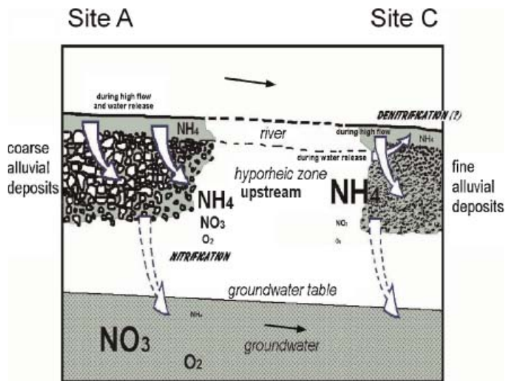
Figure 10. Conceptual model proposed for Tafna wadi surface water-ground water exchanges. This figure is available in colour online at www.interscience.wiley.com/journal/tra
