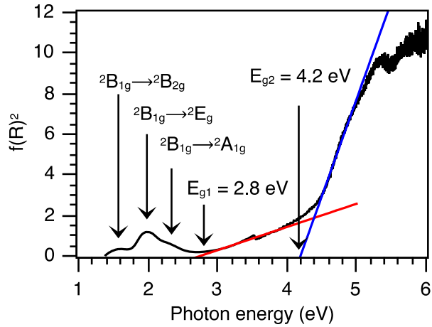
Figure 5. Optical absorption spectrum of polycrystalline \text{CaCuSi}_4\text{O}_{10} . Straight lines are linear extrapolations to determine the optical gaps E_{g,1} and E_{g,2} .
