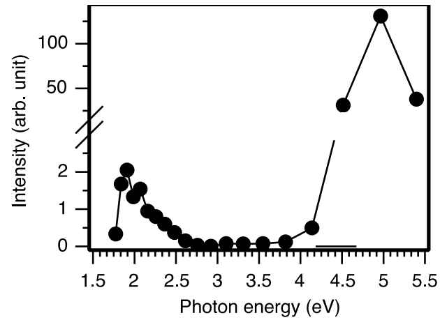
Figure 8. Excitation spectrum of the NIR luminescence at 1.45 eV in CaCuSi 4 O 10 .
