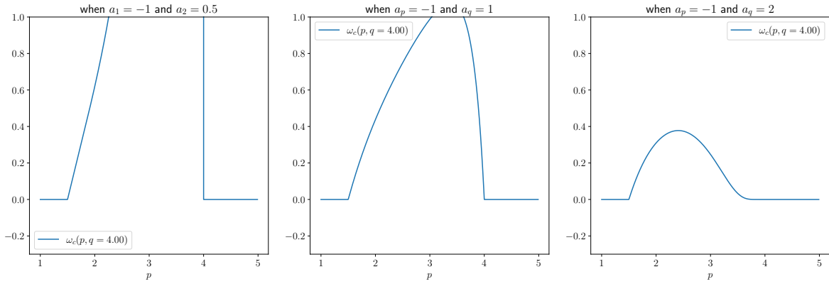
FIGURE 3. Zoom on slices of the critical surface for fixed value of q = 4
