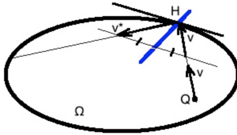
Figure 4: Projective billiard flow
