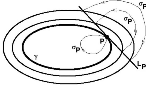
Figure 3: An integrable dual billiard structure
