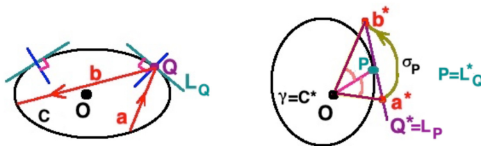
Figure 5: Euclidean billiard and its dual: Bialy – Mironov angular billiard
