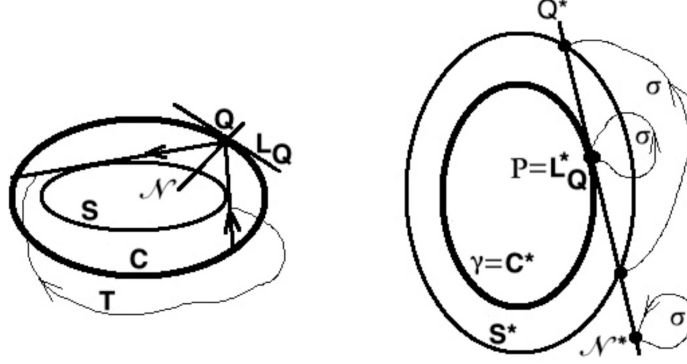
Figure 2: The projective billiard reflection involution T acting on lines through a point Q \in C and the dual involution \sigma = \sigma_P acting on the dual line Q^* tangent to the dual curve \gamma = C^* at the point P = L_Q^* .
