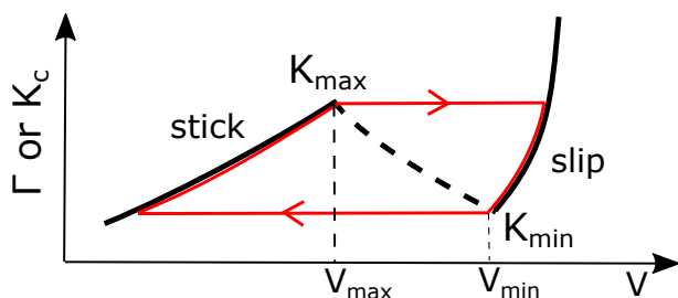
Fig. 9 Classical representation of stick-slip dynamics as a cycle (in red) on the K_C(V) curve of steady-state fracture propagation. When the applied loading rate \dot{\delta} corresponds to a steady-state velocity laying in the intermediate unstable negative slope branch (cf. Appendix), the crack propagation becomes a jerky alternation of slow and fast phases. In the slow phase (named ‘stick’) the crack propagation is so weak that K increases due to the external loading rate up to K_{max} , where the crack velocity jumps to the dynamic branch. In the fast phase (named ‘slip’) fast crack propagation over a finite crack length increment leads to sharp drop of K down to K_{min} , where the crack velocity drops.
