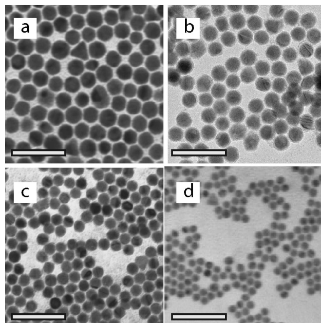
Figure 4. The size of the nanocrystal decreases from (a) to (d) as the final temperature of the solution is decreased from 280 to 240 °C. The scale bar is 100 nm.
