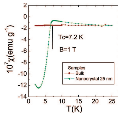
Figure 3. Magnetic susceptibility of Pb nanocrystal with diameter 25 nm, as compared to bulk Pb, under a static magnetic field of 1 T. The normal state values of magnetic susceptibility are similar, indicating that nanocrystal sample is mostly composed of metallic Pb with negligible contribution from oxide or organic ligands. Nanocrystals display the Meissner effect below the critical temperature T_c = 7.2 K, as in bulk Pb. Note that the upper critical field of bulk Pb is 0.088 T, smaller than the applied field, which explains the absence of Meissner effect in bulk Pb data.
