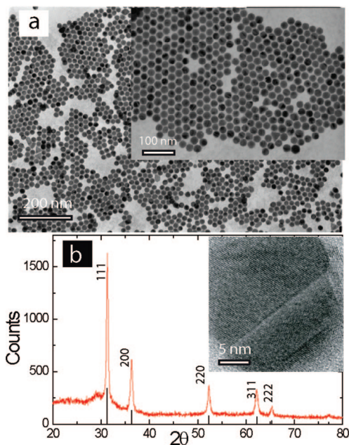
Figure 1. (a) Main panel and inset are TEM images of Pb nanocrystals obtained from two distinct synthesis. (b) Main panel: XRD pattern of the Pb nanocrystals. The standard diffraction peak positions and relative intensities of bulk FCC lead are indicated. The inset shows a HRTEM image (20 nm × 20 nm) of the nanocrystal sample. The ordered distance of 2.7 nm shown in the high-resolution image corresponds to the lattice spacing of the (111) faces of FCC Pb.
