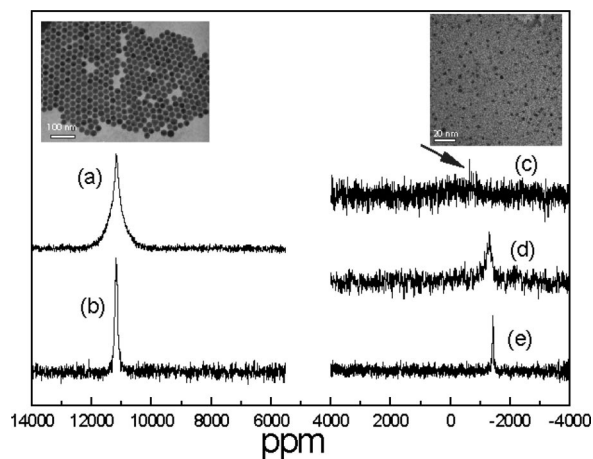
Figure 2. Pb-207 static NMR spectra of (a) metallic Pb 0 nanoparticles (left TEM picture), (b) bulk metal Pb, (c) clusters (right TEM picture), (d) lead-oleate aged under oxygen, and (e) pure lead-oleate. All of the spectra are obtained in a 7 T magnetic field at room temperature with a spin echo experiment. The position of the NMR line for lead clusters (indicated by arrow) shows that the clusters responsible for nucleation at the beginning of the synthesis are lead carboxylate aggregates.
