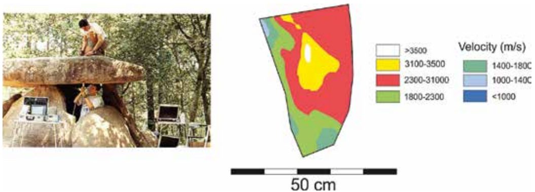
Figure 14. 3D ultrasonic tomography of the megalith d'Axeitos (Spain). Reproduced with the permission from Ebert et al. [77].
