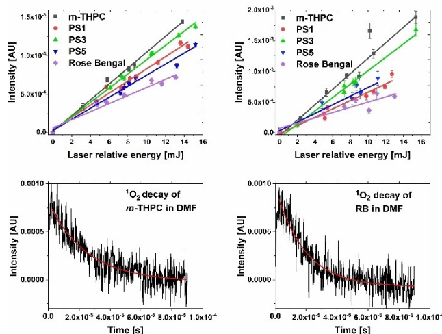
Figure 3. ^1\text{O}_2 phosphorescence intensities in DMF (top left) and DMSO (top right) as a function of the laser pulse energy. Representative ^1\text{O}_2 phosphorescence decays of m -THPC (bottom left) and Rose Bengal (bottom right) recorded in DMF.
