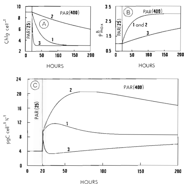
Fig. 3. Hymenomonas elongata . Theoretical approach to cellular production during a transient phase following a change in irradiance from PAR(25) to PAR(400). (A) Changes in Chl a cell -1 with 3 different kinetic constants; (B) changes in P b max with 2 kinetic constants; (C) changes in cellular production in accordance with changes in Chl a cell -1 and P b max (curves numbered as those for Chl a cell -1 and P b max ). Values used in simulations are listed in Table 5
