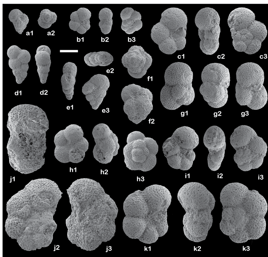
Figure 3. SEM images of planktic foraminiferal index-species and other relevant species (scale bar = 100 microns). (a) Guembelitra cretacea (364-M0077A-39R-2 85–86 cm); (b) Parvularugoglobigerina eugubina (364-M0077A-40R-1 17–18 cm); (c) Parasubbotina pseudobulloides (364-M0077A-39R-1 128–129 cm); (d) Chiloguembelina morsei (364-M0077A-39R-2 98–99 cm); (e) Chiloguembelina midwayensis (364-M0077A-39R-3 41–42 cm); (f) Globoconusa daubjergensis (364-M0077A-37R-2 116–117 cm); (g) Subbotina triloculinoides (364-M0077A-38R-2 60–61 cm); (h) Eoglobigerina edita (364-M0077A-38R-2 60–61 cm); (i) Globanomalina compressa (364-M0077A-37R-1 116–117 cm); (j) Praemurica uncinata (364-M0077A-37R-1 96–97 cm); (k) Praemurica inconstans (364-M0077A-37R-2 37–38 cm).
