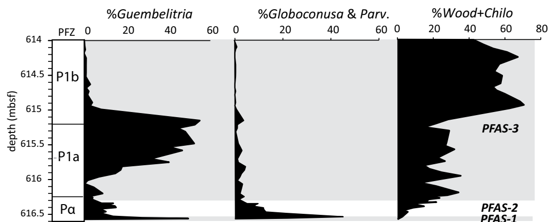
Figure 7. Quantitative stratigraphic distribution of early Danian planktic foraminiferal groups at Site M0077 and Planktic Foraminiferal Acme Stages (PFAS) 1–3: PFAS-1 is the predominance of Guembelitra , PFAS-2 is the predominance of Parvularugoglobigerina and Globoconusa (or Palaeoglobigerina according to Arenillas & Arz, 2017), and PFAS-3 is the predominance of Woodringina and Chiloguembelina . A second acme of Guembelitra (or Chiloguembelitra according to Arenillas & Arz, 2017) occurs within this stage across the Tethys, as is also evident at Site M0077.
