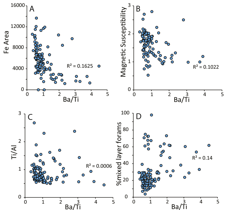
Figure 8. Cross plots of Ba/Ti ratios (i.e., export productivity) with proxies for stratification and terrigenous flux: (a) XRF Fe counts, a proxy for sedimentary dilution by terrigenous sediments, (b) magnetic susceptibility, a proxy for the influx of terrigenous material, (c) Ti/Al, a proxy for the relative abundance of aeolian (Ti) versus riverine (Al) flux, (d) the percent abundance of mixed layer foraminifera versus total foraminifera, a proxy for the vertical stratification of the upper water column. R^2 values (and your eyeballs, probably) indicate that all four are uncorrelated and thus changes in export productivity were not related to terrigenous flux or water column stratification.
