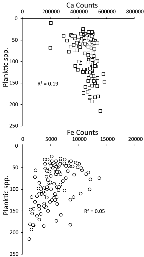
Figure 5. Preservation versus calcium and iron XRF counts. Better preservation is toward zero on the y-axis (i.e., fewer unidentifiable foraminifera). Two outliers >80,000 from pyrite-rich samples at the base of the section were removed from the Fe plot. Ca shows a weak negative correlation with good preservation while Fe shows a weak positive correlation with good preservation. This pattern is the opposite of trends caused by dissolution.
