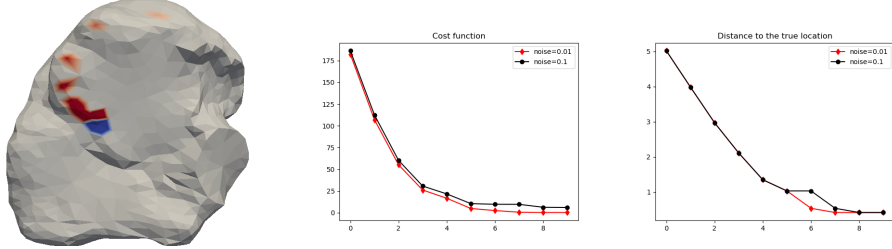
FIGURE 7. Left: location of the successive iterates x^k (red) and the true source point x^* (blue). Center: evolution of the cost function J . Right: evolution of the distance to the solution \|x^k - x^*\| in both cases.
