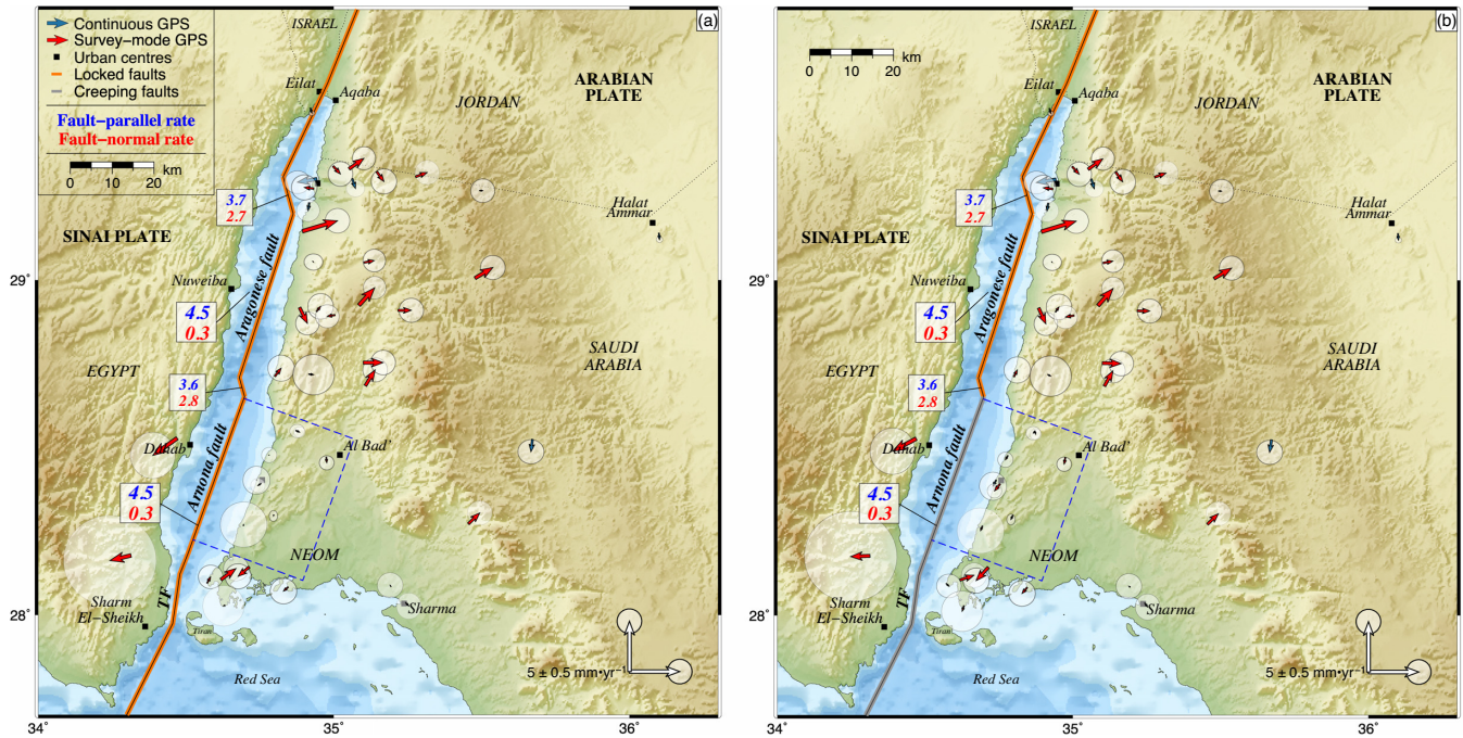
Figure 6. Panel (a) shows residual velocities after implementing the first back-slip model scenario assuming full interseismic locking on all the fault traces. Panel (b) shows the residuals obtained after implementing the second scenario assuming full creep along the Arnona fault and the TF. Orange and grey lines represent locked and creeping fault traces, respectively. Residual rates of seven near-fault stations within the blue dashed boxes are analysed in Fig. S6 in the Supporting Information.
