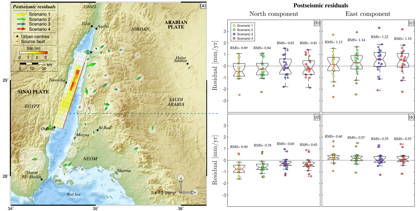
Figure 10. Residual velocities after implementing four post-seismic model scenarios discussed in the text, with the orange line delineating the 1995 coseismic fault rupture of the Aragonese fault (after Baer et al. 2008). For visualization purpose, 95 per cent confidence ellipses are shown only for the best-fitting post-seismic model (scenario 2). The contrast between the residuals of stations in the northern half of the gulf (East of the Aragonese fault trace) and South (East of the Arnona fault trace) is illustrated in panels (b)–(e), with notched boxes enclosing data within 25th and 75th percentiles. For each scenario, the median of the misfit distribution is shown as a solid red line and whiskers extend to the most extreme data points not considered as outliers, which are represented by the red crosses.
