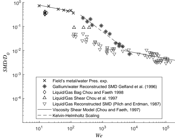
Figure 16: Dimensionless SMD as function of We number. Dark symbols are for liquid-liquid cases and open symbols are for gas-liquid cases. Correlations based on power law analysis are depicted.
