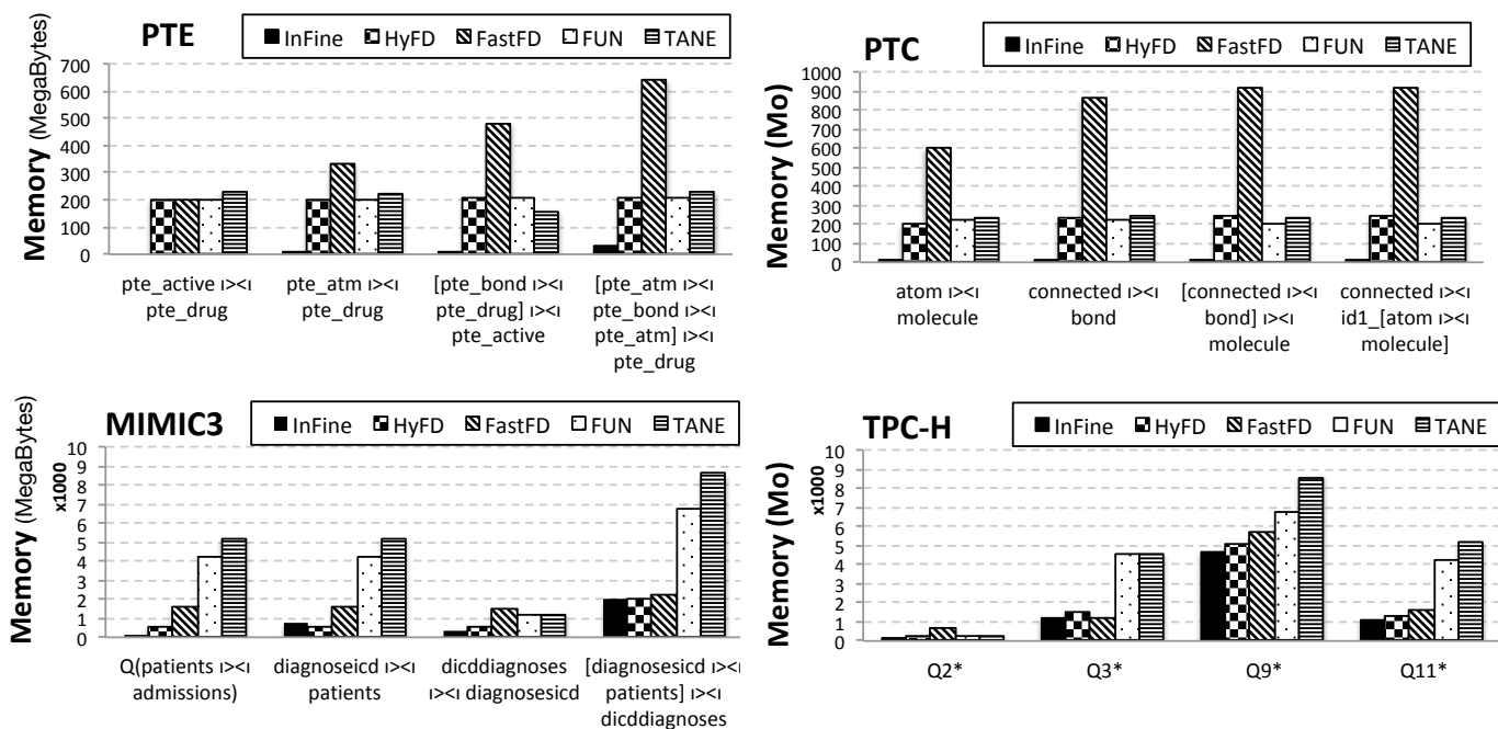
Fig. 4: Maximal memory consumption (in MegaBytes) of InFine against HyFD, FastFDs, FUN, and TANE algorithms
