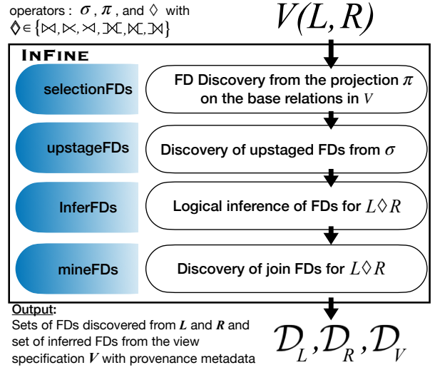
Fig. 2: Workflow of InFine for discovering inferred FDs from a view specification V(L, R)
