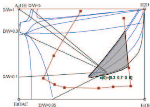
Figure 18. Still paths calculated with different production ratios.
