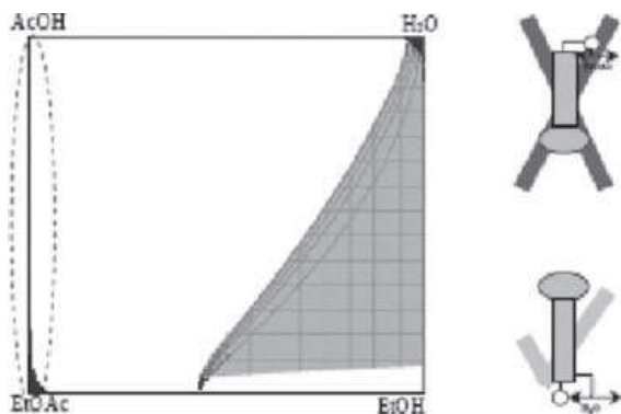
Figure 10. Feasible region of the reactive sections.
