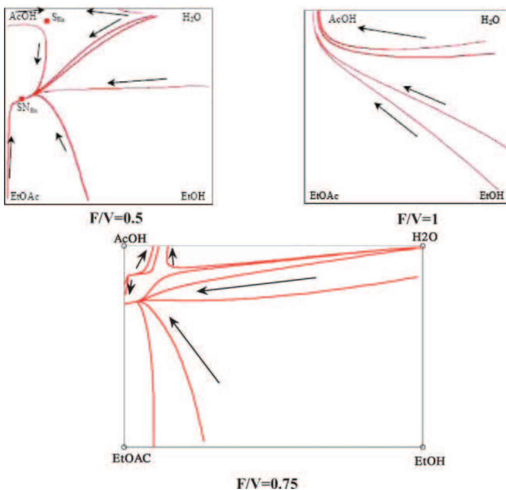
Figure 15. Reactive extractive profiles, at R = 10 .
