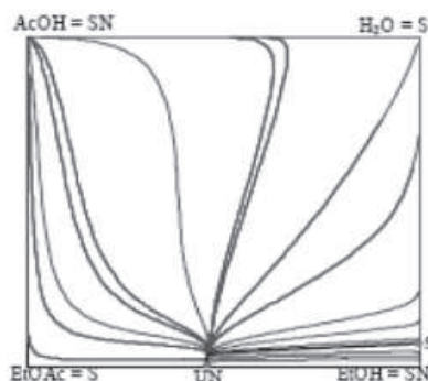
Figure 7. Residue curves maps of the studied system.
