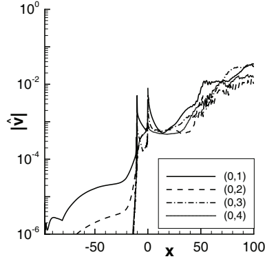
Fig. 26 Maximum amplitude of the normal velocity v for steady modes (0,k) .
