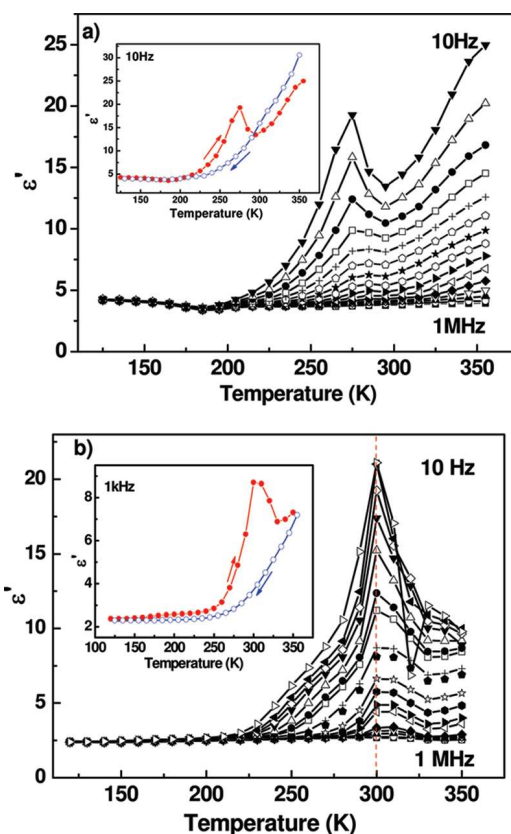
Figure 4. Temperature dependence of the real part of the complex dielectric permittivity of \text{Rb}_{0.8}\text{Mn}[\text{Fe}(\text{CN})_6]_{0.93} \cdot 1.62\text{H}_2\text{O} (a) and \text{Co}_3[\text{W}(\text{CN})_6]_2(\text{pyrimidine})_4 \cdot 6\text{H}_2\text{O} (b) recorded at different frequencies in the heating mode. The hysteresis curves at selected frequencies are shown in the inserts.
