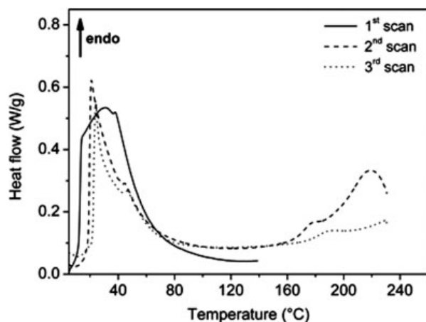
FIGURE 1 DSC thermograms of powdered exon 6 at first (solid line), second (dash line) and third (dot line) scan.
