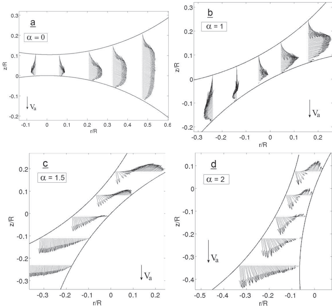
Figure 7. Velocity field in the gap between the beads ( e=R/10 , Re=29 ). Frontal and oblique approach: (a) \alpha=0 , (b) \alpha=1 , (c) \alpha=1.5 , (d) \alpha=2 .
